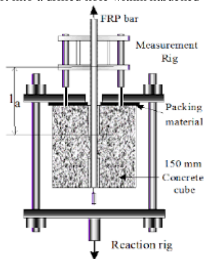
Fig.3 Pull-Out Test
