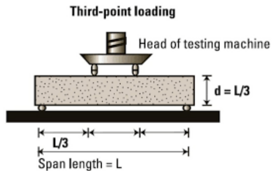
Fig. 2 Flexural Test
