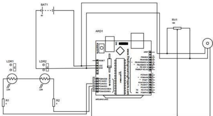
Fig Circuit
