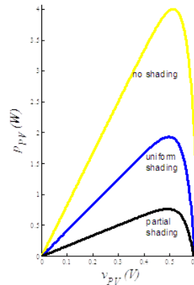
Fig 7 P-V plot for shading and partial shading
