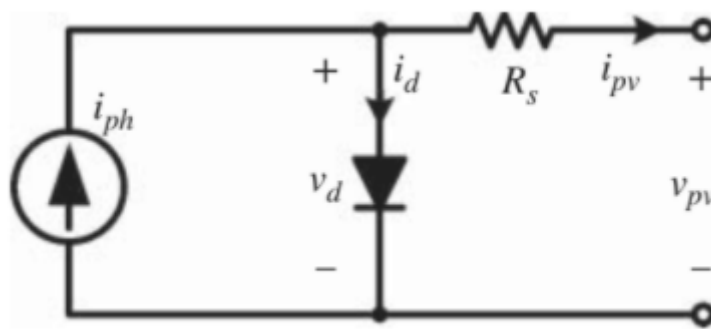
Fig. 1: Equivalent circuit of PV cell using single diode model.
