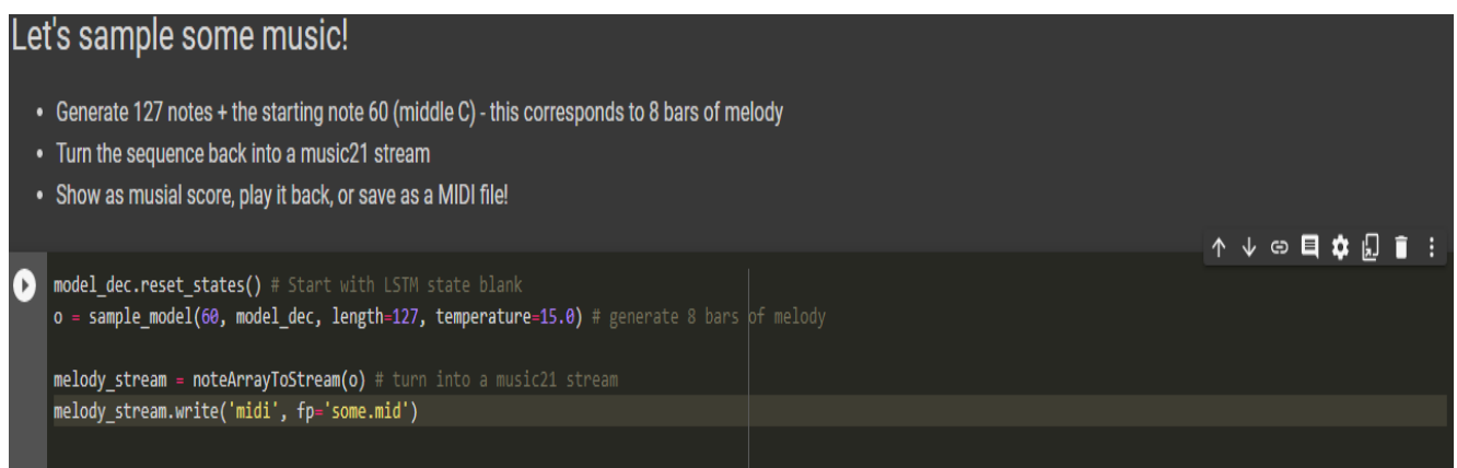
Figure 1: Music Generation
