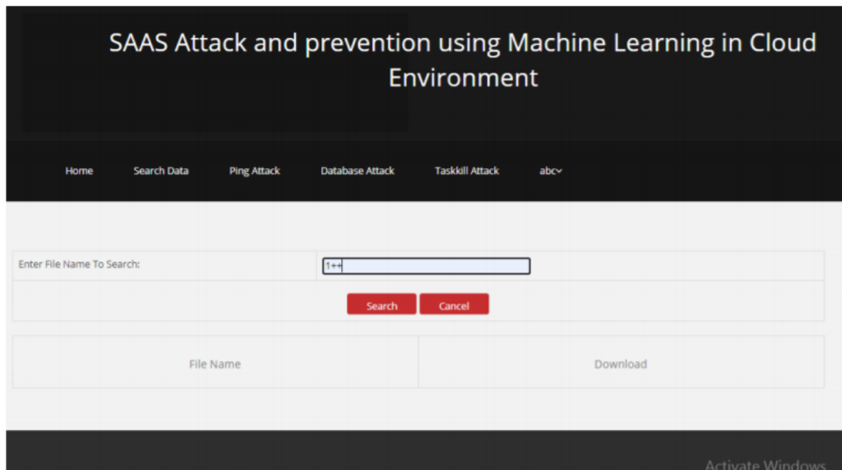
Figure 2 : File search
