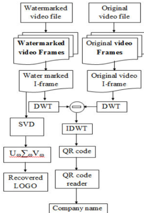
Figure 2 Block diagram of the extracting process
