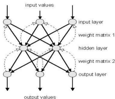
Fig. 2) Back propagation Network Testing of query images :
