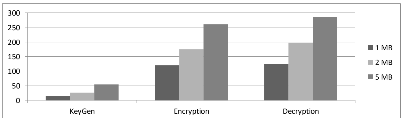
Figure 3 :Data encryption performance base on data size
