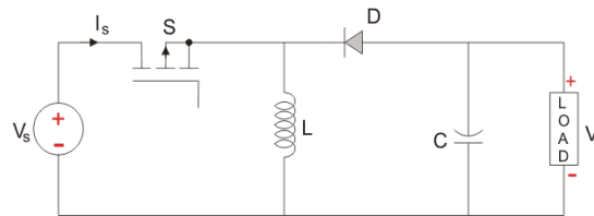
Fig 1: Configuration for buck-boost converter
