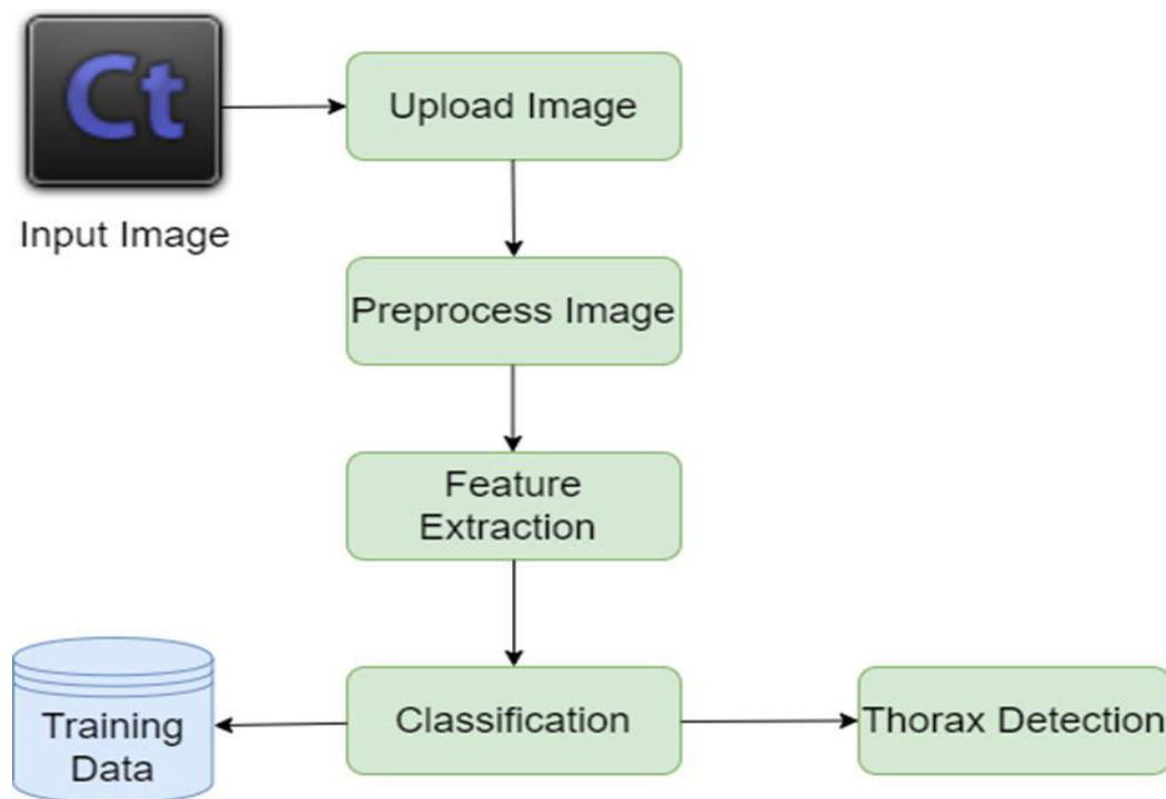
Figure 1. System Architecture
