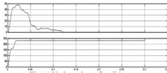
Fig.(c) Under voltage Condition Fig:-Under voltage of three phase induction motor.
