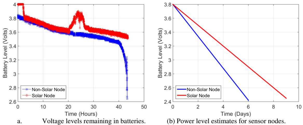
Fig. 3: Power results for the proposed system.
