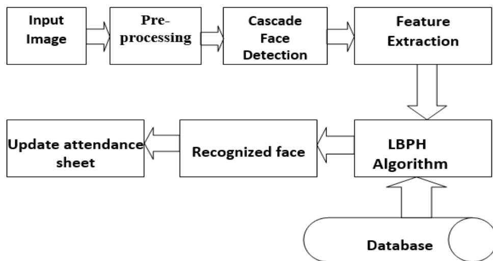
Fig .1. Block diagram of Face Recognition Process
