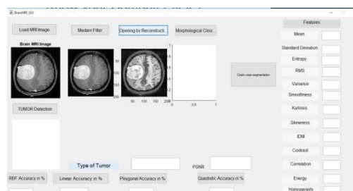
Figure 5: opening by reconstruction
