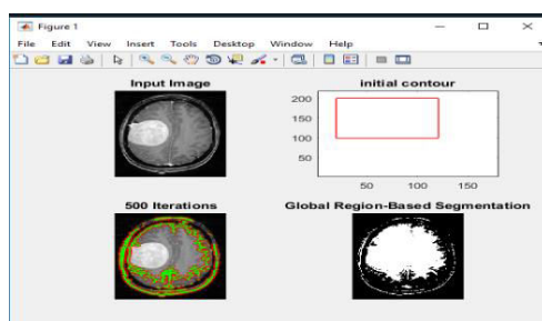
Figure 7: Chain-void segmentation
