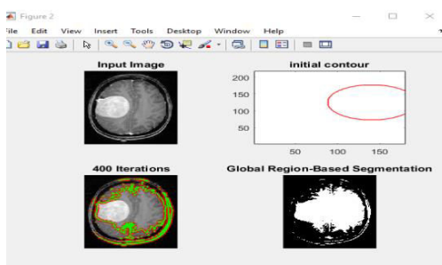
Figure 8: Tumor Detection
