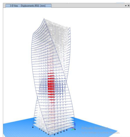
Figure1.8: 2.5 Degree Displacement due to dead load
