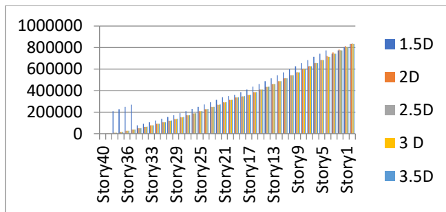
Graph1.9: Maximum Overturning Moment
