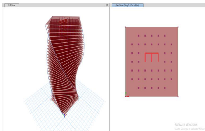
Figure1.10: Plan & 3D View of 3.5 Degree
