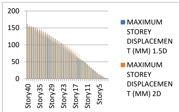
Graph: Story Displacement
