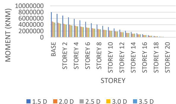
OVERTURNING MOMENT (KNM)
