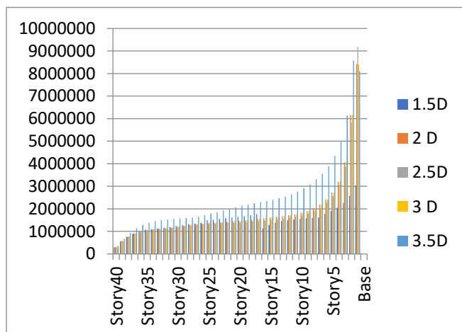
Graph1.10: Maximum Story Stiffness
