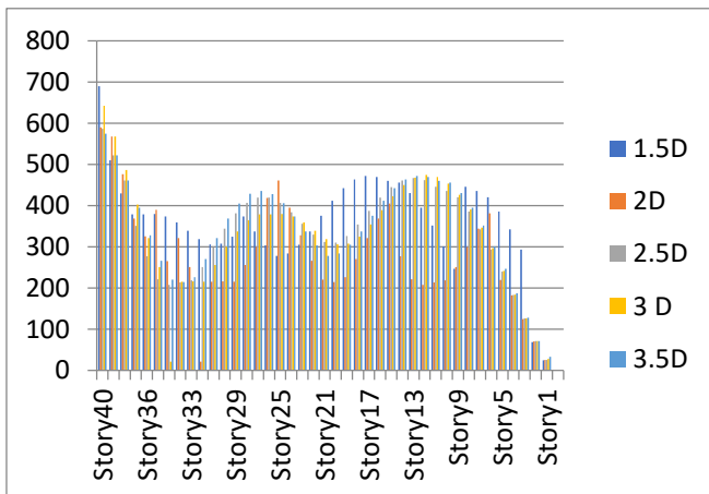
Graph: Maximum Storey Accelerations (Mm/Sec 2 )
