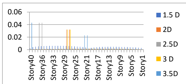
Graph: Maximum Story Drift
