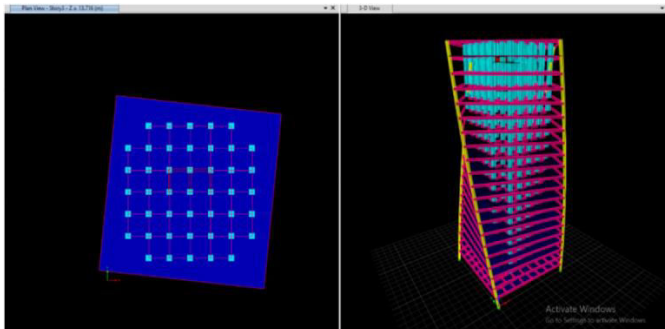
Figure 1.3: 2.5 Degree Model design
