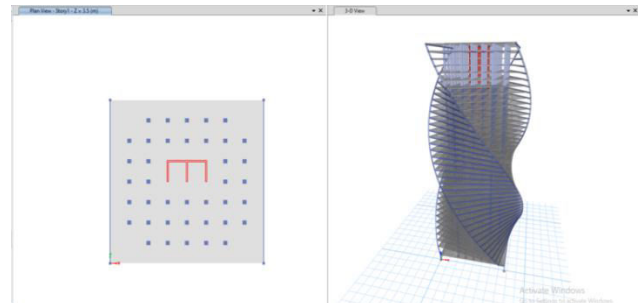
Figure4.6: 1.5 Degree Plan & 3D View
