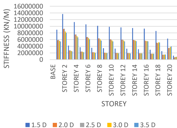
STOREY STIFFNESS (KN/M)
