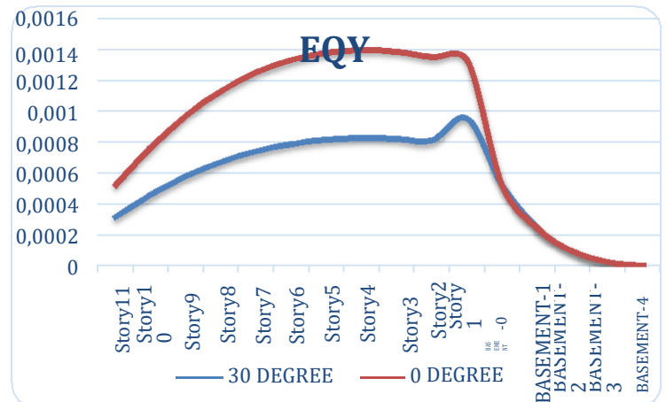
Figure 11- lateral loads of EQY
