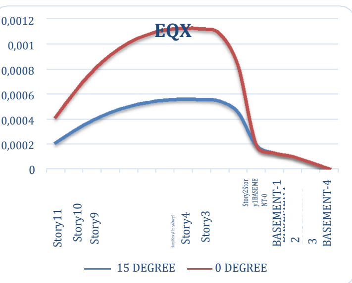
Figure 6- storey drift of EQX
