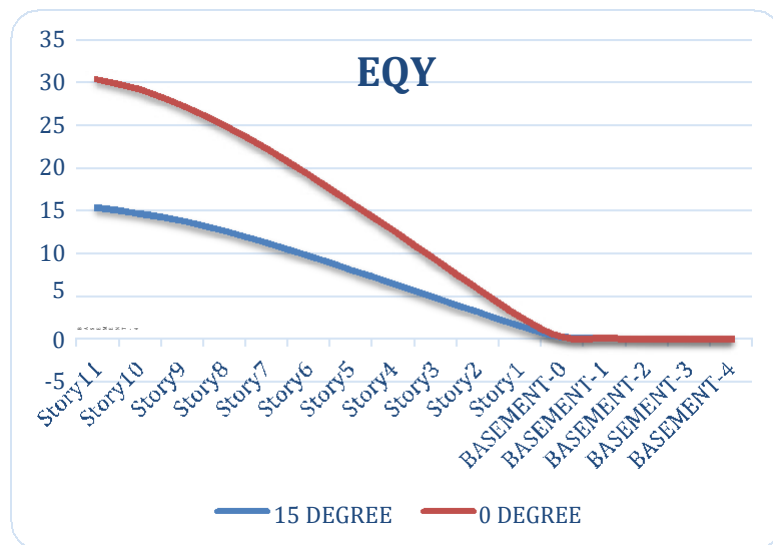
Figure 3 – Displacement of EQY
