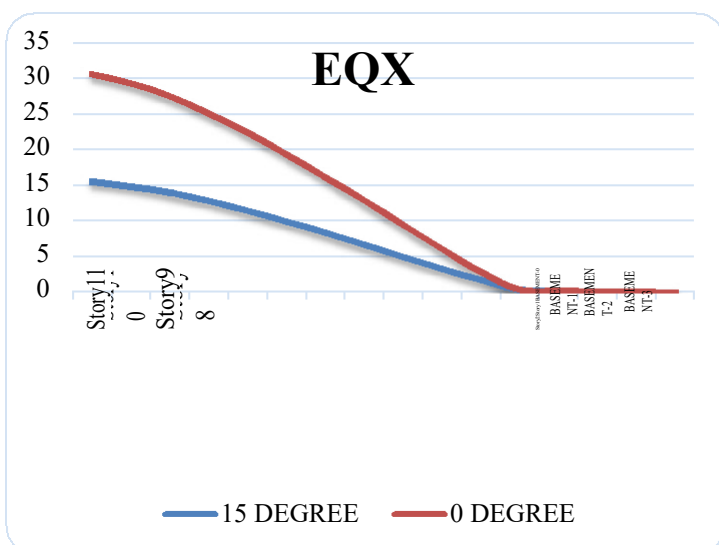
Figure 2 – Displacement of EQX
