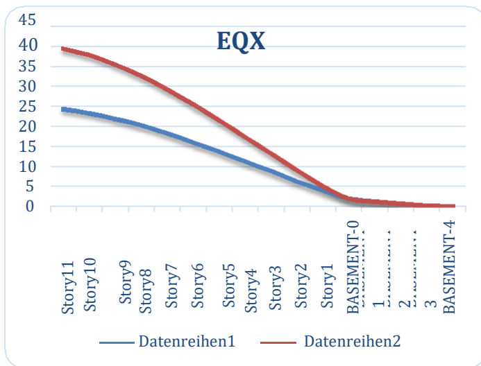
Figure 8- displacement of EQX
