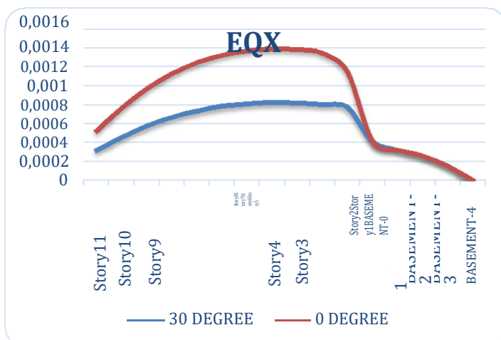
Figure 10- lateral loads of EQX
