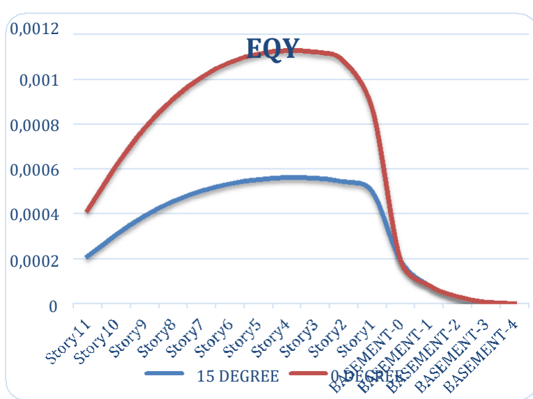
Figure 7- storey drift of EQY
