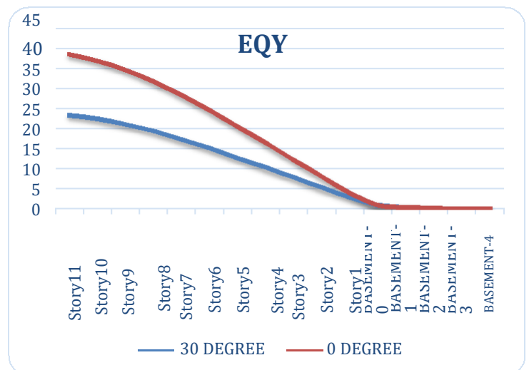
Figure 9- displacement of EQY
