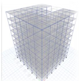
C- SHAPE G+10 BUILDINGS
