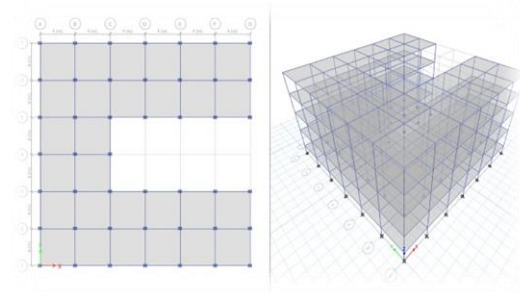
C- SHAPE G+5 BUILDINGS
