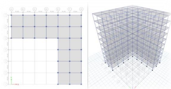
L- SHAPE G+10 BUILDINGS
