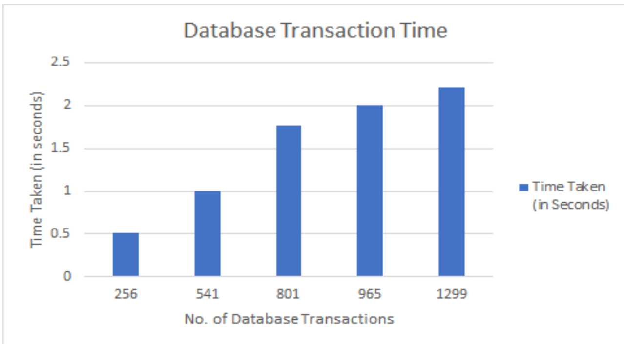
Figure 2: Blockchain Transactions
