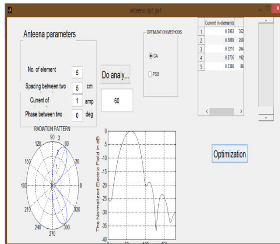
Figure 7 the performance of antenna parameter with genetic algorithm
