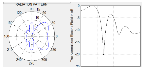
Fig-3 The optimization of radition pattenen with number of element N=5 and desired Direction for main beam is 30 degree with PSO method
