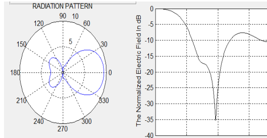
Fig-5 The optimization of radiation pattern with number of element N=5 and desired Direction for main beam is 20 degree with PSO method.
