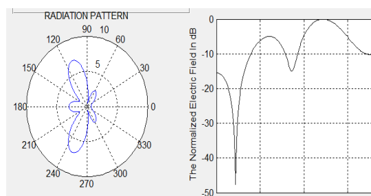
Fig-4 The optimization of radition pattenen with number of element N=5 and desired Direction for main beam is 120 degree with PSO method
