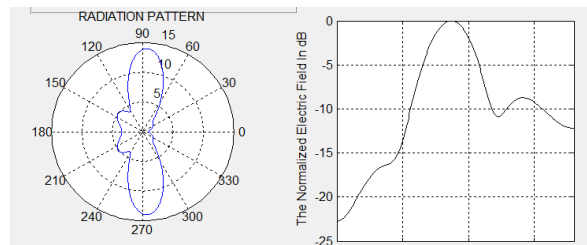
Fig-2 The optimization of radition pattenen with number of element N=5 and desired Direction for main beam is 90 degree with PSO method
