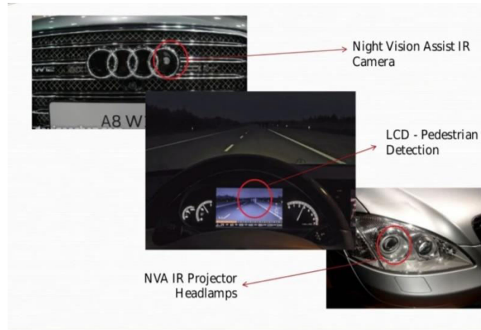
Fig 4:- Vision Enhancement System
