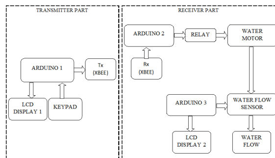
Figure 1.1: Block Diagram
