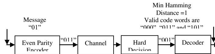
Fig. 1: Block Diagram of Error Detecting Codes
