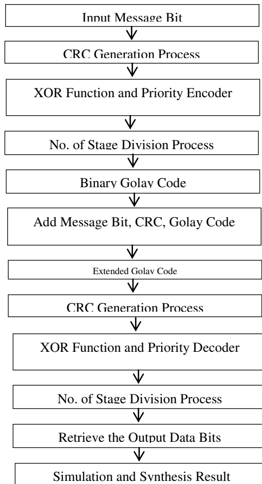
Fig. 4: Flow Chart of Golay Encoder and Decoder
