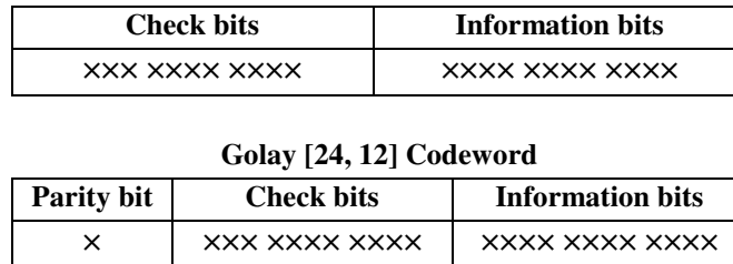
Fig. 3: Block Diagram of Golay Code
