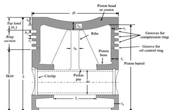
Figure 1: Schematic diagram of Piston
