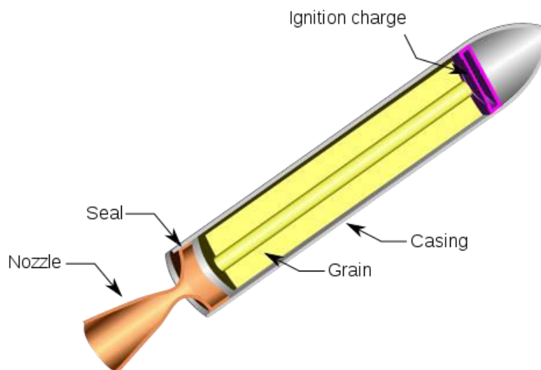
FIGURE 1 PARTS OF THE SOLID FUEL ROCKET
