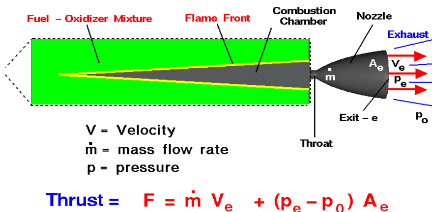
Figure 3 Working principle of the solid fuel rocket
