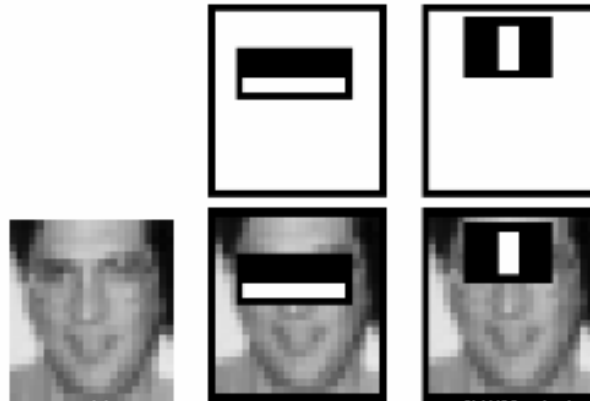
Figure 3.3: Image Processing
