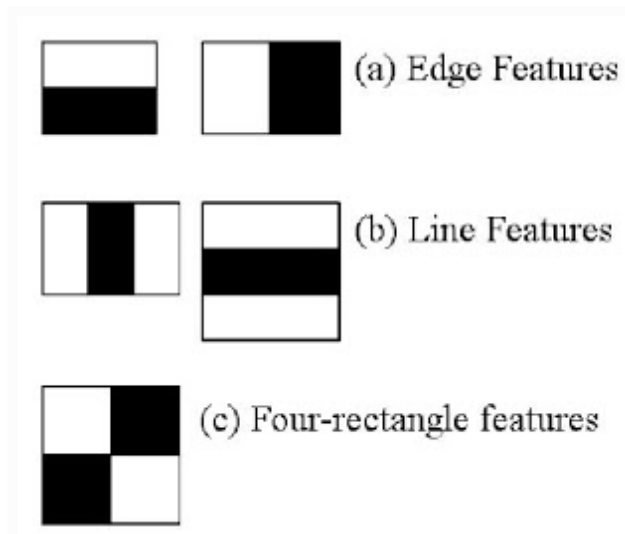
Figure 3.2: Problem Analyses
