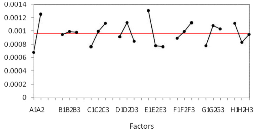
Figure 1: Response Graph for MRR
