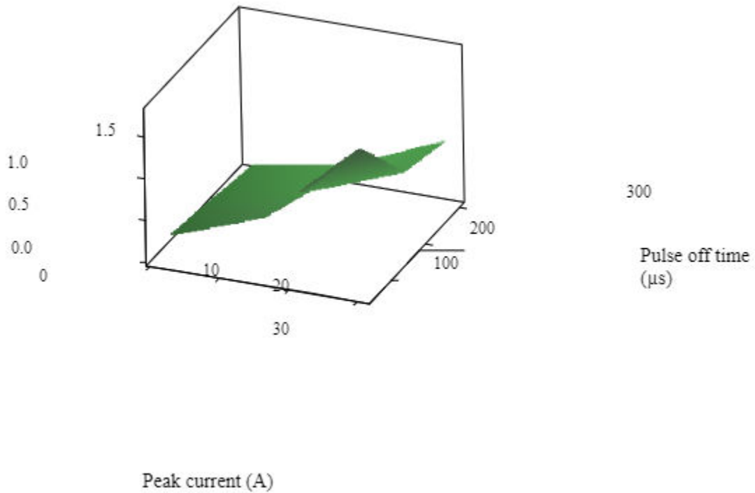
Figure 5: 3-D surface plot of the effect of peak current and pulse off time on MRR.
