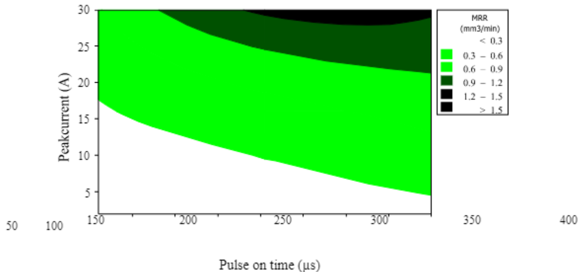
Figure 2: 2-D contour plot of the effect of peak current and pulse on time on MRR.
