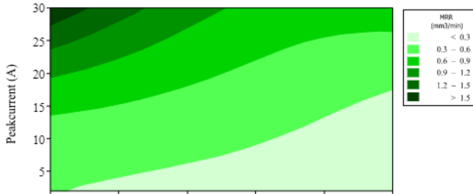
Figure 4: 2-D contour plot of the effect of peak current and pulse off time on MRR.
