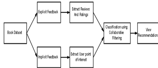
Figure 1. System Architecture
