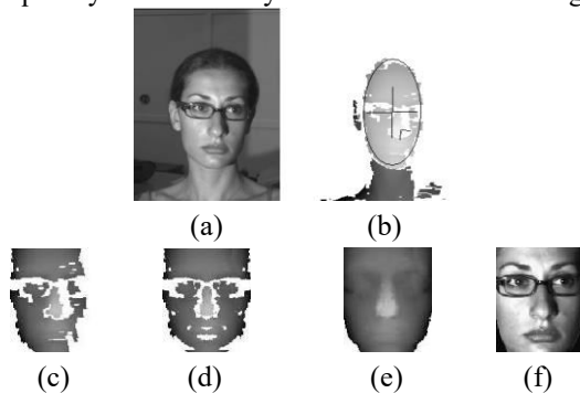
Fig. 1. Pose compensation example. (a) Original color image, (b) original depth image showing detected head blob and estimated local coordinate system fixed on the nose, (c) rectified depth image, (d) symmetry-based interpolation, (e) final linear interpolated depth image, (f) rectified color image.
