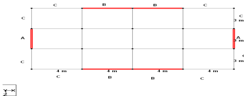
Figure 2 Plan of building showing location of braced frame & shear wall frame
