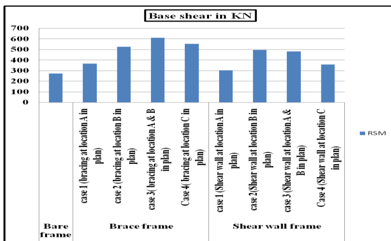
Graph 1 Design Base Shear in KN
