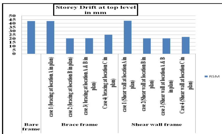
Graph 4 Storey drift in mm
