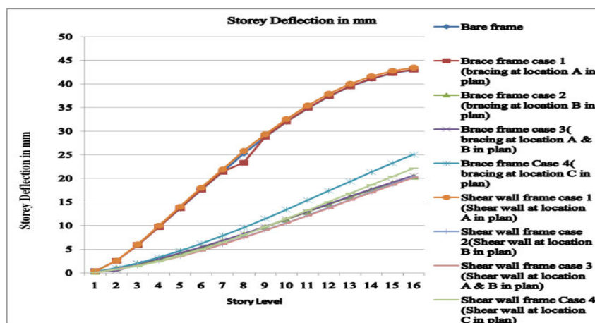
Graph 3 Storey deflection in mm
