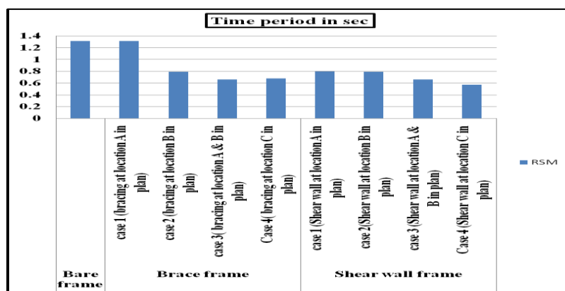
Graph 2 Time period in sec
