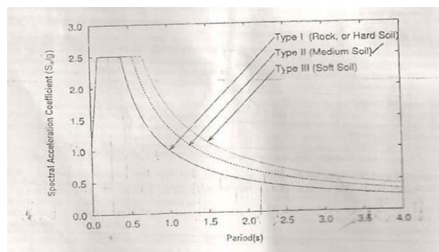
Figure3 Response Spectrum for soil as per IS1893 part-I (2002)
