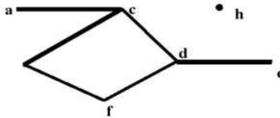
Figure (3.1) undirected G
