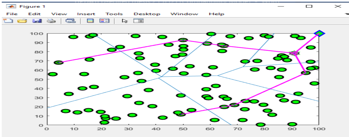
Figure 4.4 : Nodes Structure
