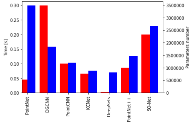
Fig 9. Comparison of the model complexity
