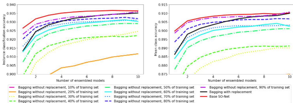
Fig 11. Class accuracy Vs Number of Ensemble models
