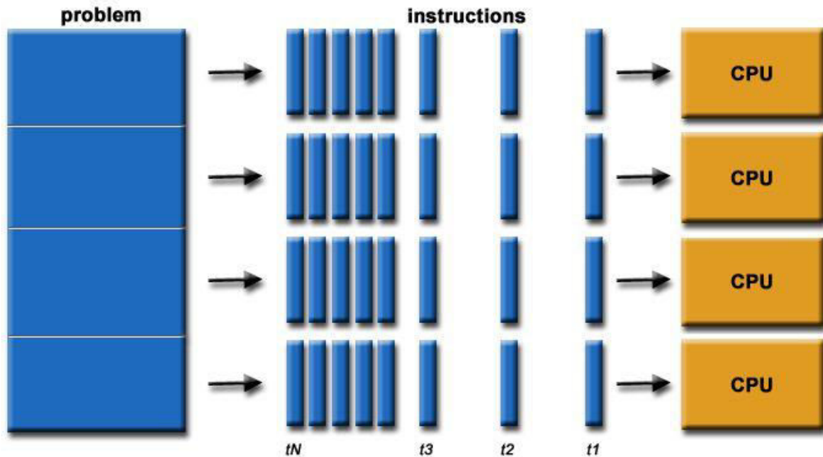
Fig 1.17-Diagrammatic representation of parallel computing
