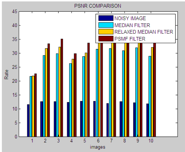
Fig 4.7:- PSNR evaluation
