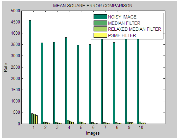
Fig 4.6:- Mean Square Error Evaluation
