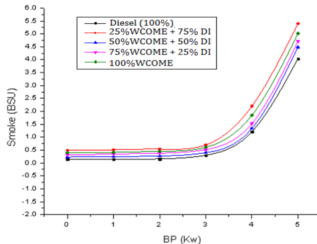
Fig.5. Smoke Vs Break Power
