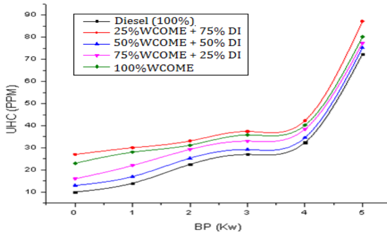
Fig.5. Un-Burnt Hydro Carbon Vs Break Power
