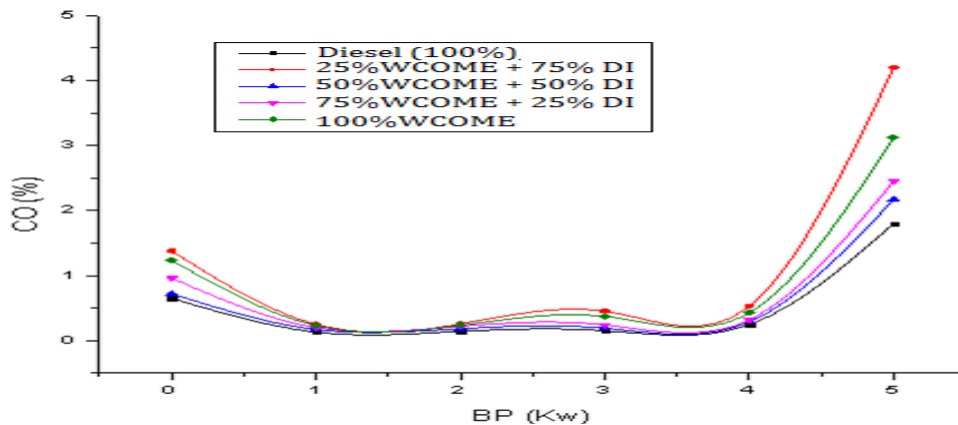
Fig.4. Carbon Monoxide Vs Break Power
