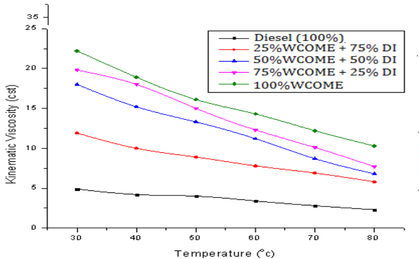
Fig.3. Viscosity Vs Temperature
