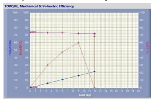
Fig. 6. Load vs. Mechanical & Volumetric Efficiency
