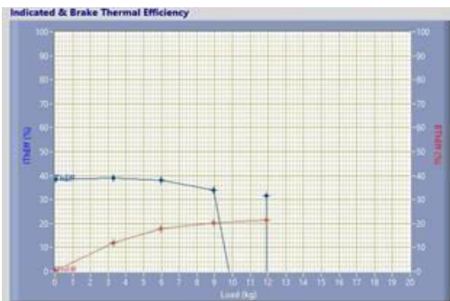
Fig. 4. Load vs. Indicated & Thermal Efficiency
