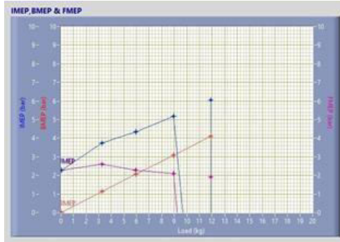
Fig. 3. Load vs. IMEP, BMEP & FMEP
