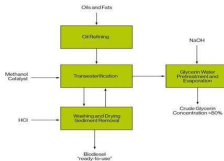
Fig. 1. Transesterification process
