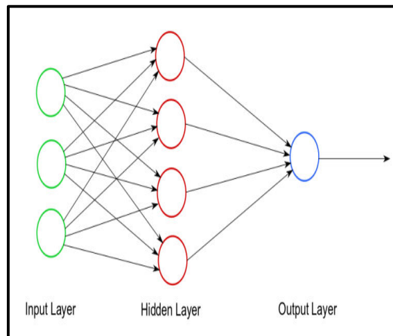
Figure 2: RNN Layers
