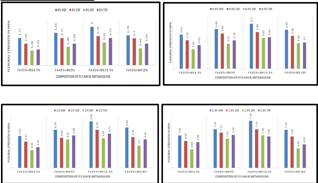
Fig 9. Flexural strength results for FA+MK mixes without any inclusion of steel fibers, Fig 10. Flexural strength results for FA+MK mixes reinforced with 0.5% HSF, CSF, SSF & TSF, Fig 11. Flexural strength results for FA+MK mixes reinforced with 1% HSF, CSF, SSF & TSF, Fig 12. Flexural strength results for FA+MK mixes reinforced with 1.5% HSF, CSF, SSF & TSF
