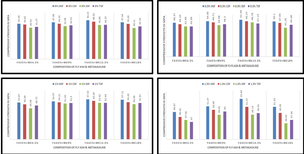
Fig 1. Compressive strength results for FA+MK mixes without any inclusion of steel fibers, Fig 2. Compressive strength results for FA+MK mixes reinforced with 0.5% HSF, CSF, SSF & TSF, Fig 3. Compressive strength results for FA+MK mixes reinforced with 1% HSF, CSF, SSF & TSF, Fig 4. Compressive strength results for FA+MK mixes reinforced with 1.5% HSF, CSF, SSF & TSF
