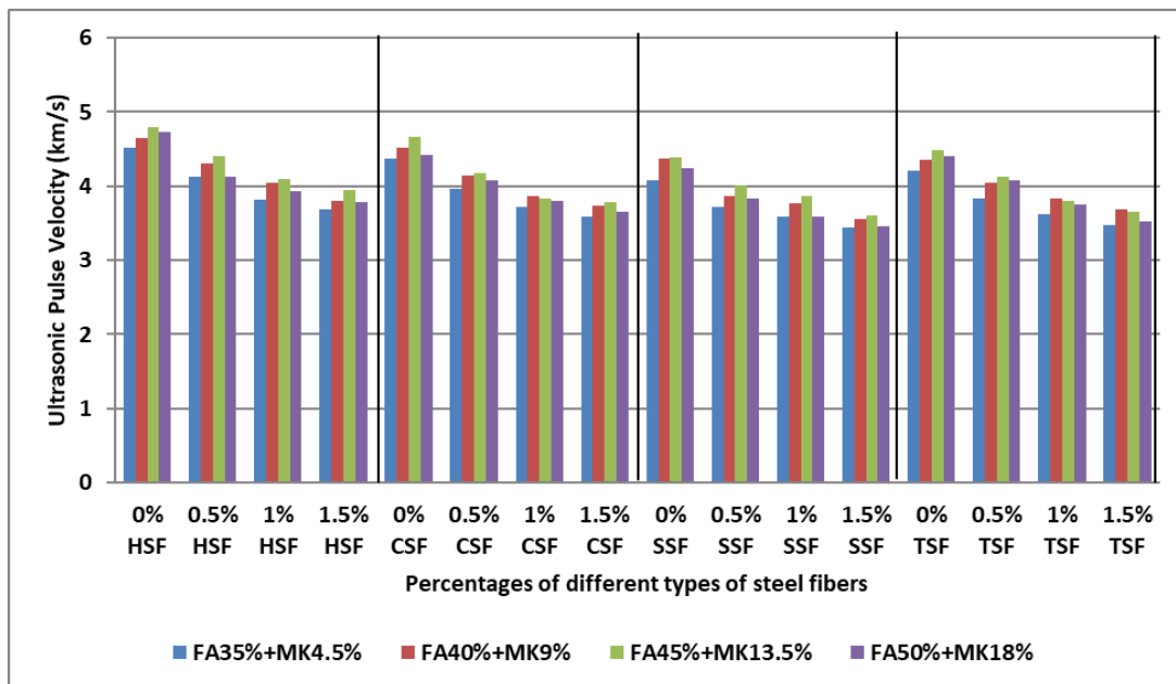
Fig 18. Cumulative graph showing the variations in UPV results for all concrete compositions included with different fractions of HSF, CSF, SSF & TSF
