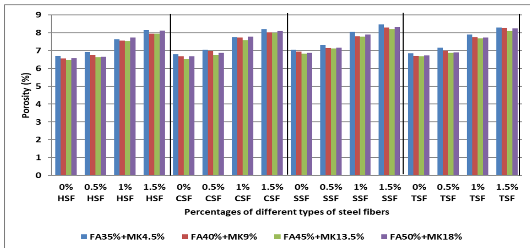
Fig 17. Cumulative graph showing the variations in porosity results for all concrete compositions included with different fractions of HSF, CSF, SSF & TSF
