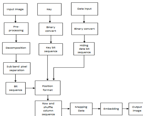
Fig.3: Proposed System Block Diagram at Encryption
