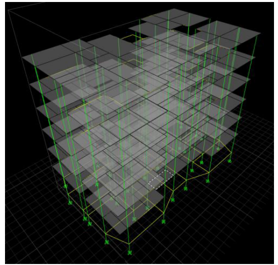
3D Model from Etabs
