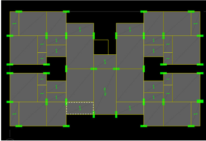
2D Plan from Etabs
