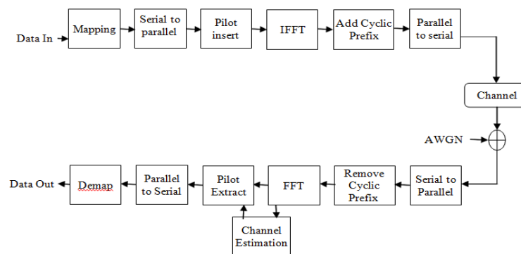
Fig. 1: Block Diagram of OFDM with Channel Estimation
