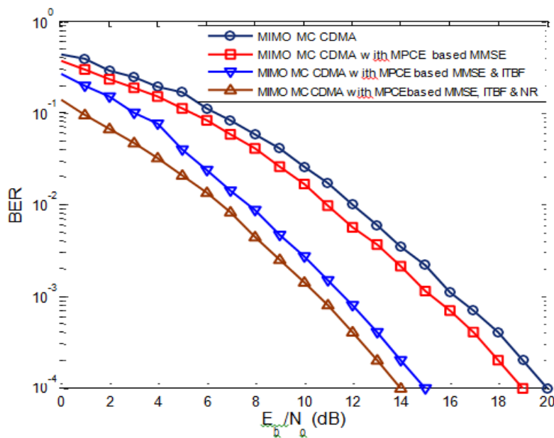
Fig. 4: Execution of 2 x 1 x 2 receiving wire setup for 16 QAM
