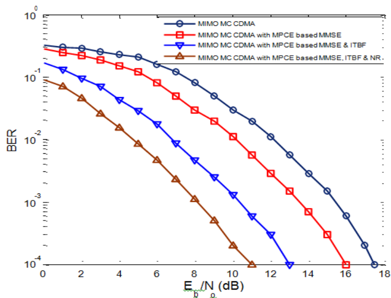
Fig. 6: Execution of 4 x 1 x 4 receiving wire setup for 16 QAM
