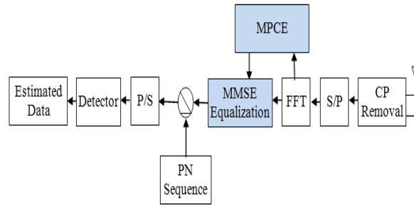
Fig. 2: Block Diagram of MIMO System with PN Sequence
