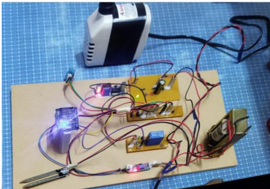
Fig 2: Microcontroller Connection
