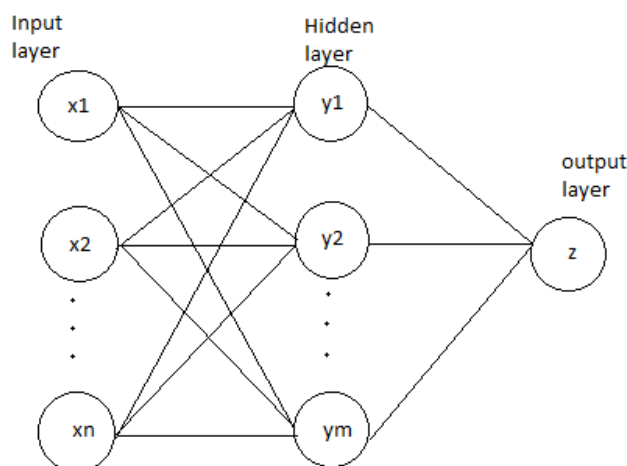
Fig. 1 Neural Network
