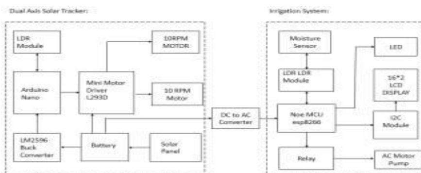
Fig 1. Smart Irrigation systems Using Dual Axis Solar Tracker
