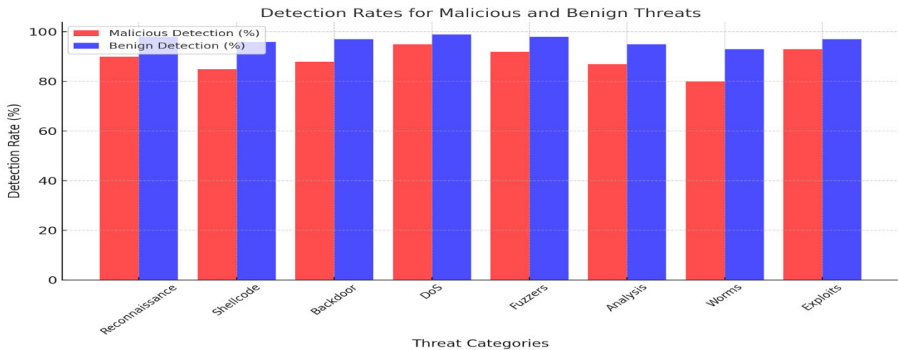
Fig. 1 Model Performance
