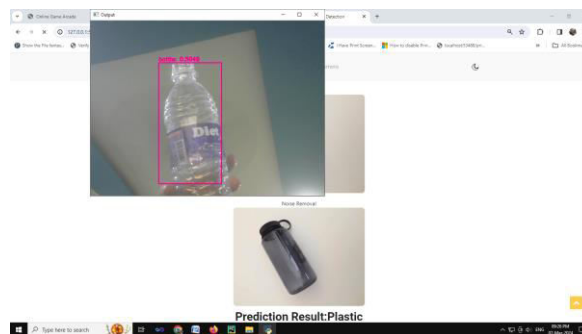
Fig 7: Trash classification
