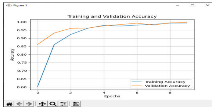
Fig 4: Training accuracy
