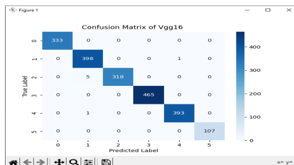
Fig 5: Confusion matrix
