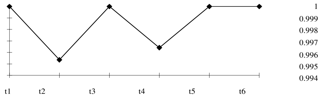
Figure 2: Variation by term Table 3. Score and rank for each DMUs
