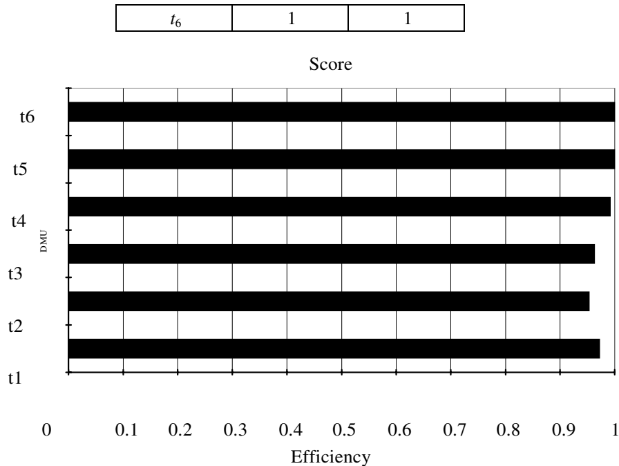
Figure 3: Score for each DMUs
