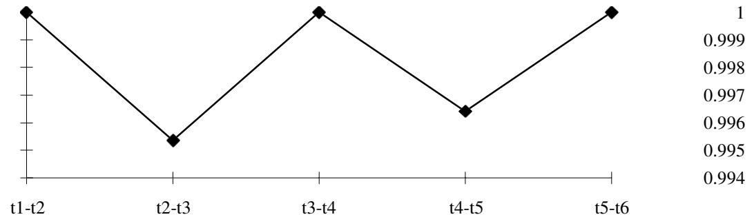
Figure 1: Variation through Window
