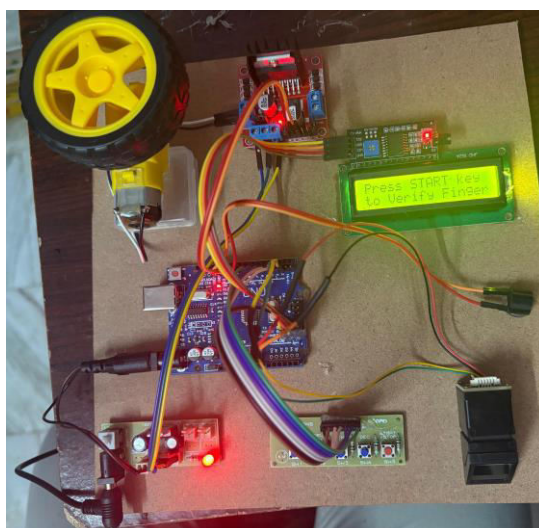
Fig 7.1. System Waiting for Verify the Finger
