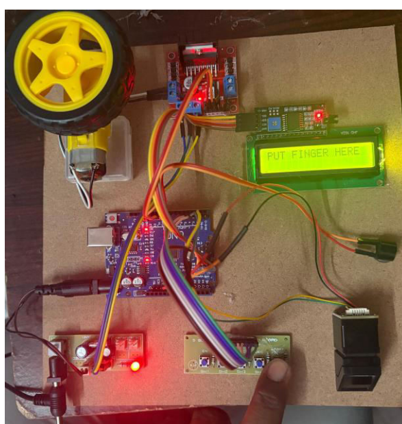
Fig 7.2. System Verify the user Finger
