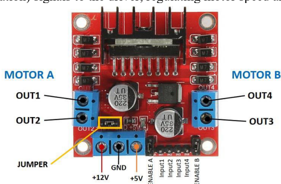
Fig. 3.2.4. L298N Motor Driver
