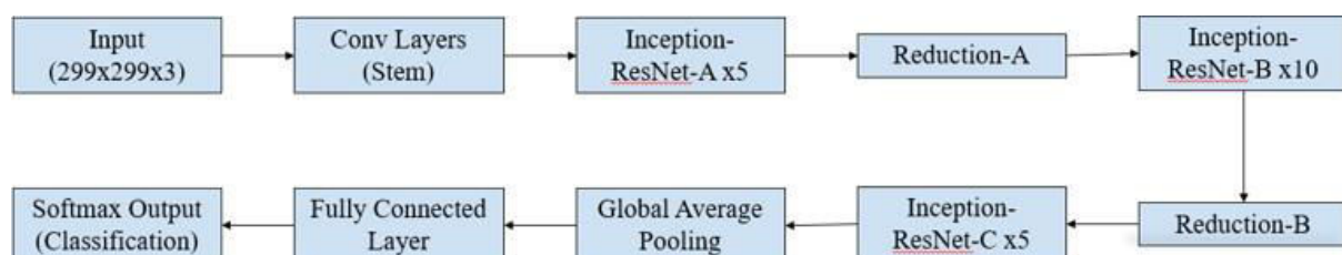
Figure 3: Architecture of Inception-V3 Model
