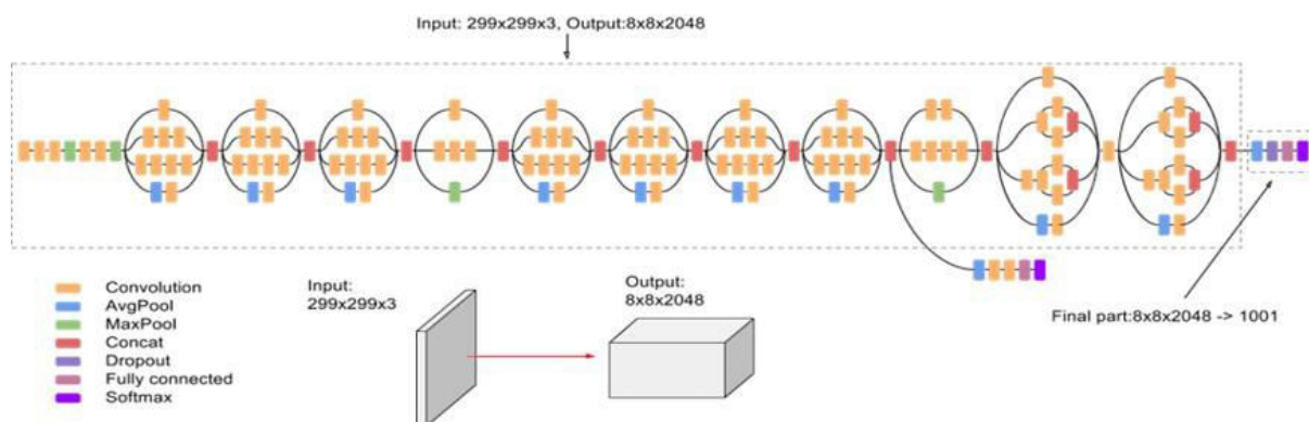
Figure 2: Architecture of Inception-ResNet-V2 Model
