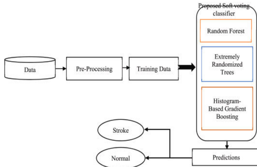
Figure 3: Soft Voting Classifier
