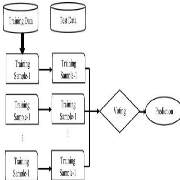
Figure 4 : Random Forest Classifier
